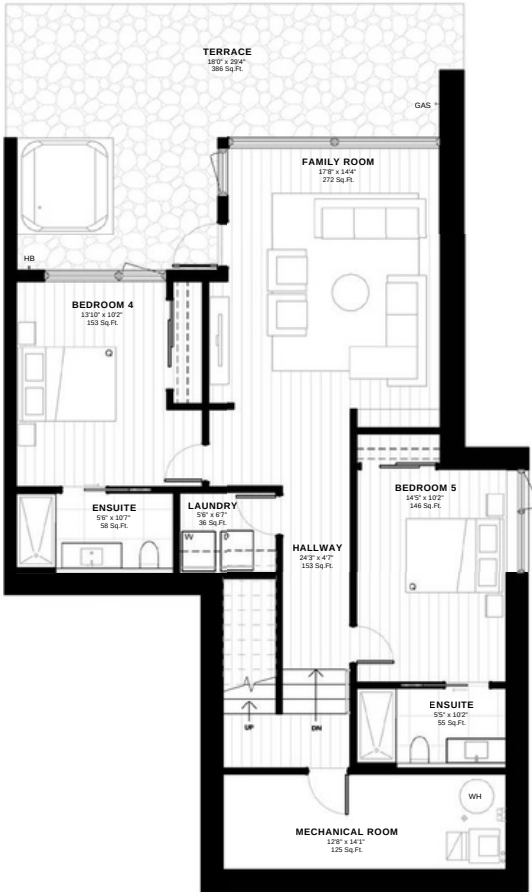
BASEMENT FLOOR 1147 SQ FT + 176 SQ FT MEC
